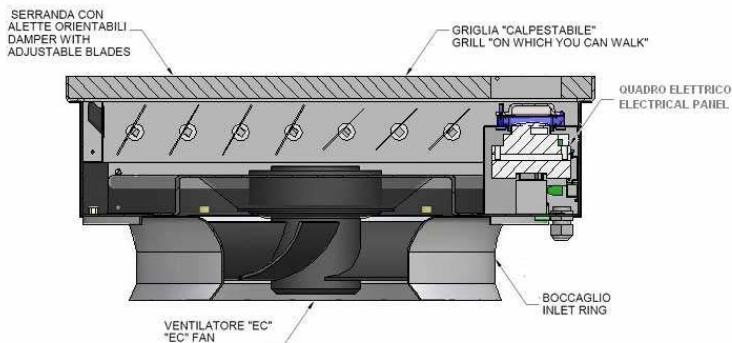
- section of active floor module integrated in the floor -
